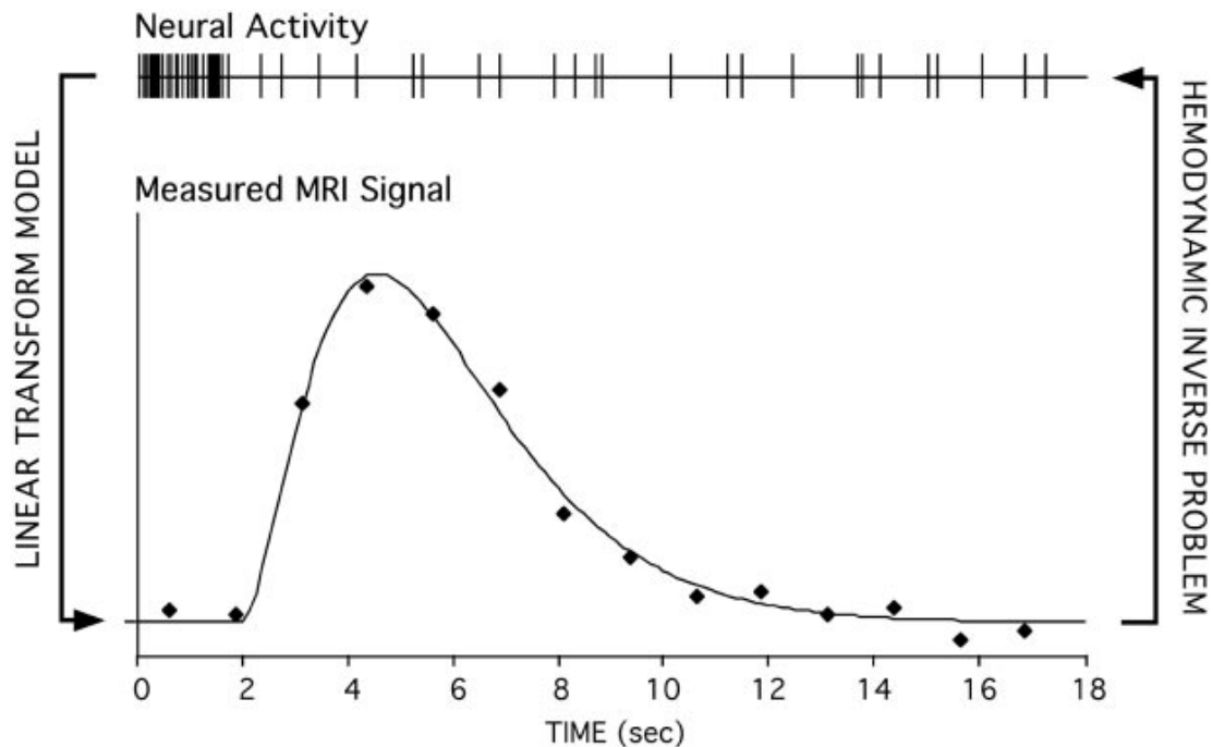
Fig. 1. A schematic illustrating the linear transform model that specifies the relation between averaged neural activity and the temporally prolonged hemodynamic response measured by fMRI. The inverse transformation presents the hemodynamic inverse problem. From “The Hemodynamic Inverse Problem: Making Inferences About Neural Activity From Measured MRI Signals”, by R.L. Buckner, 2003, Proceedings of the National Academy of Sciences , 100(5), p. 2178. Copyright 2003 by National Academy of Sciences, U.S.A. Reprinted with permission.
